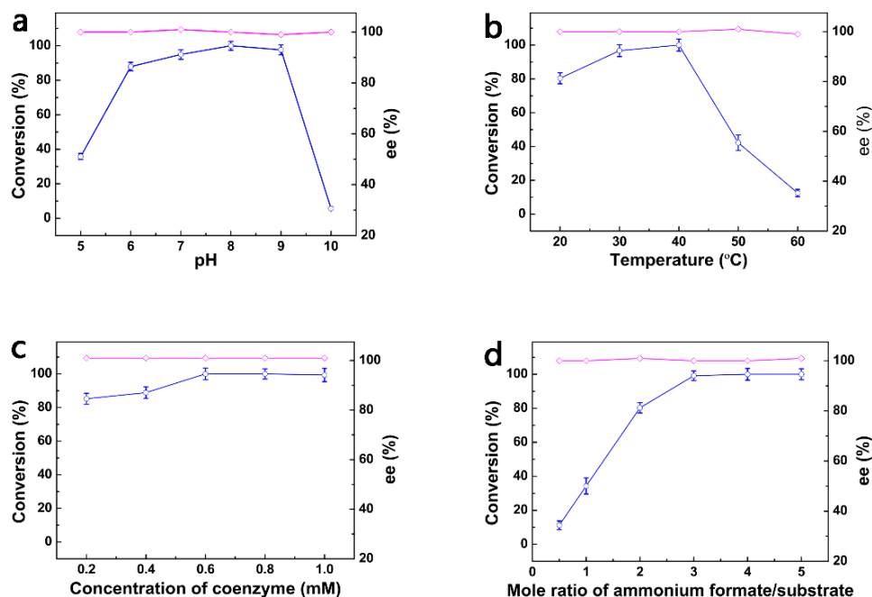
Figure 7. The effects of pH (a), temperature (b), the cofactor concentration (c) and the mole ratio of ammonium formate to substrate (d) on the biocatalytic performance of whole-cell biocatalysts.
