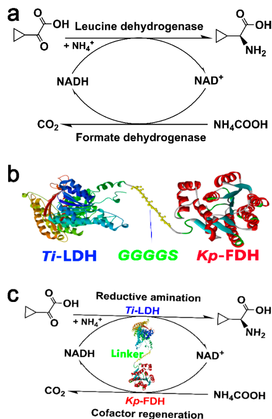
Figure 2. (a) Enzyme-coupled biocatalytic process for the synthesis of ( S )-2-cyclopropylglycine and cofactor regeneration. (b) Construction of bifunctional enzyme, and (c) Bifunctional enzyme-mediated asymmetric synthesis of ( S )-2-cyclopropylglycine and cofactor regeneration.
