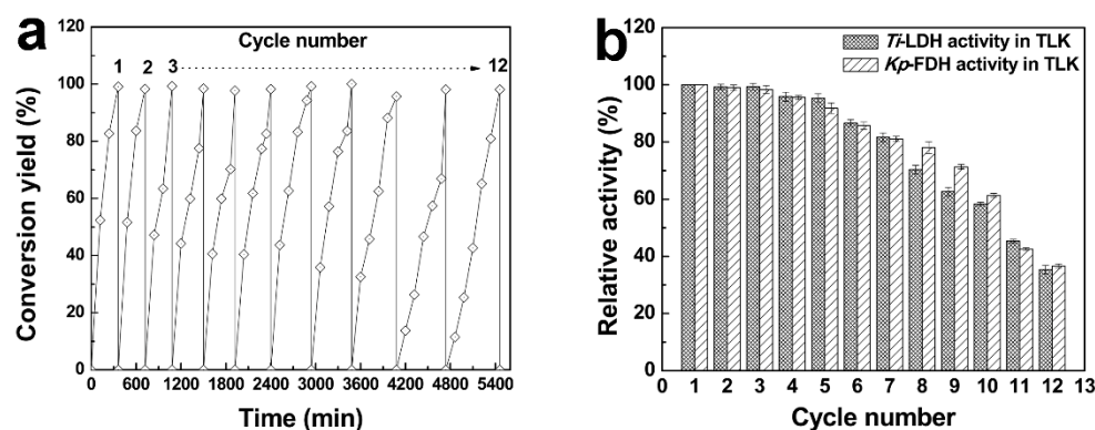
Figure 9. (a) Continuous synthesis of (S)-cyclopropylglycine. When the last cycle was completed, the dialysis tube containing E. coli (TLK) cell lysates was directly transferred to a new reaction medium, indicative of the start of the next one. The reaction was continued for 12 cycles. (b) Relative activity of Ti -LDH and Kp -FDH in TLK.
