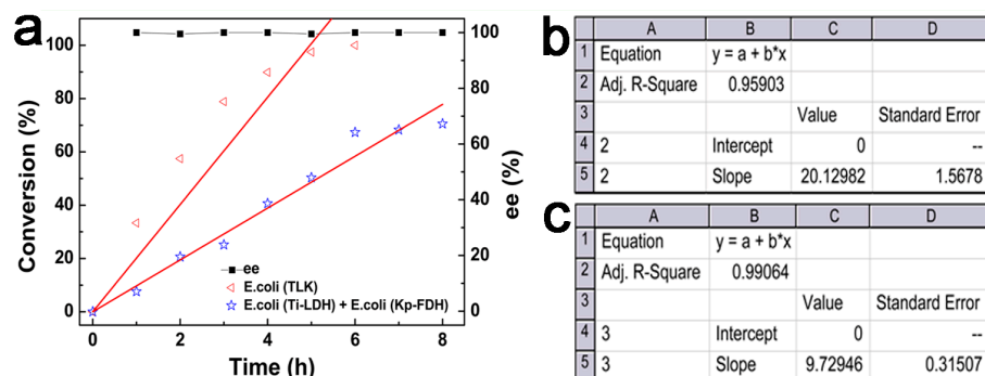
Figure 6. (a) Biocatalytic synthesis of (S)-cyclopropylglycine catalyzed by a combination of E. coli (Ti-LDH) and E. coli (Kp-FDH) and a self-sufficient whole-cell E. coli (TLK). The slopes of the straight lines represented the overall rate of (S)-cyclopropylglycine using a combination of E. coli (Ti-LDH) and E. coli (Kp-FDH) (c) and E. coli (TLK) (b), respectively.
