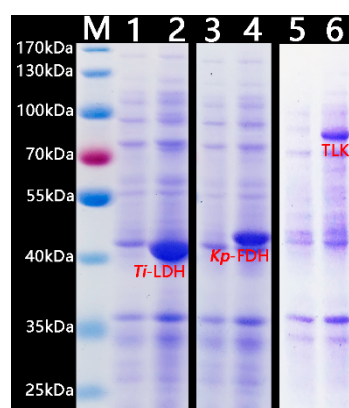
Figure 3. 12% SDS-PAGE analysis of Ti -LDH, Kp -FDH, and TLK expression. Lane M, protein molecular weight markers. Lane 1, 3, 5, and Lane 2, 4, 6, the E. coli cell lysate induced before and after 0.4 mM IPTG for E. coli ( Ti -LDH), E. coli ( Kp -FDH), and E. coli (TLK), respectively.
