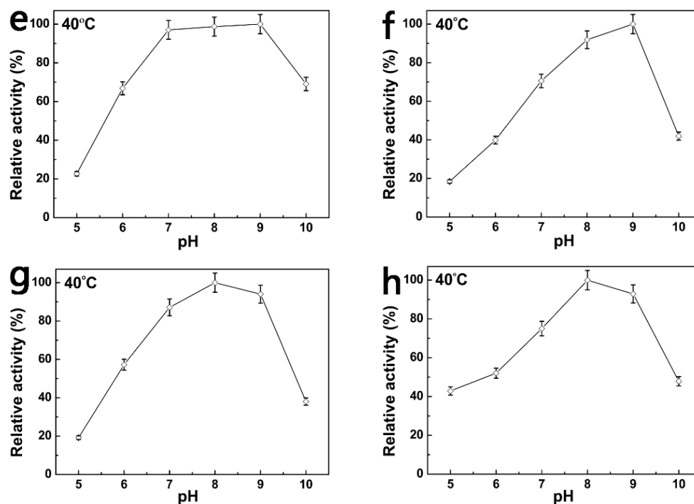
Figure 4. The effects of temperature and pH on the activities of Kp -FDH (a,e), Ti -LDH (b,f), cofactor regeneration enzyme ( Kp -FDH domains) (c,g) and carbonyl reductive amination ( Ti -LDH domains) (d,h) in the bifunctional enzyme TLK.
