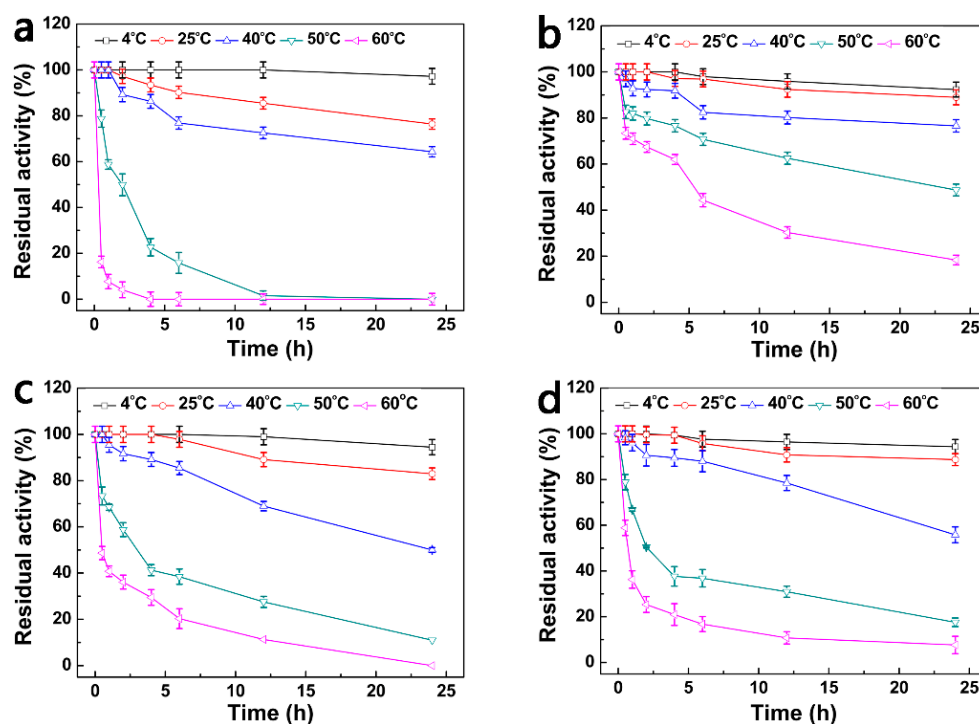
Figure 5. Thermostability of Kp -FDH (a), Ti -LDH (b), cofactor regeneration enzyme ( Kp -FDH domains) (c) and carbonyl reductive amination ( Ti -LDH domains) (d) in TLK.
