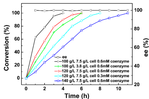
Figure 8. The time course of reductive amination of potassium cyclopropylglyoxylate to produce (S)-cyclopropylglycine in the presence of coenzyme at 40 °C and pH 8.0.
