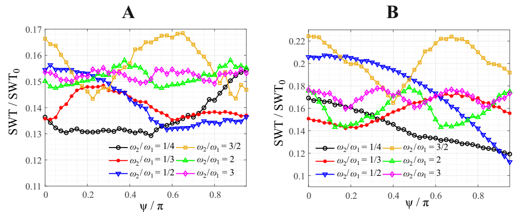
Figure 4. Normalized maximum SWT parameter for the different-frequency bimodal contact oscillation between a paraboloid and a flat, as a function of the phase angle \psi , for different values of the frequency ratio. (A): \delta_A = 0.25 \delta_0 ; (B): \delta_A = 0.75 \delta_0 .
