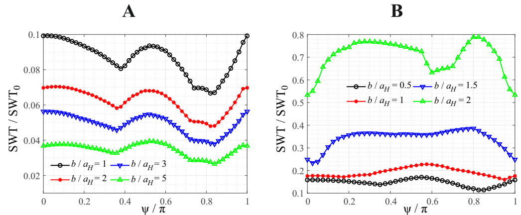
Figure 5. Normalized maximum SWT parameter for the same-frequency bimodal contact oscillation between a flat face indenter and a flat, as a function of the phase angle \psi , for different values of the radius of the punch face. (A): rounded flat punch; (B): truncated paraboloid.
