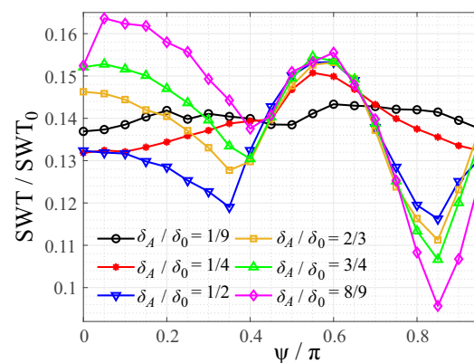
Figure 3. Normalized maximum SWT parameter for the same-frequency bimodal contact oscillation between a paraboloid and a flat, as a function of the phase angle \psi , for different values of the normal oscillation amplitude.
