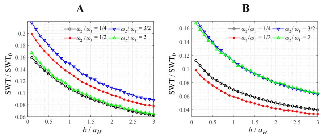
Figure 6. Normalized maximum SWT parameter for the different-frequency bimodal contact oscillation between a rounded flat punch and a flat, as a function of the normalized radius of the punch face b/a_H , for different values of the frequency ratio between tangential and normal oscillation. (A): phase angle \psi = 0 ; (B): phase angle \psi = \pi .
