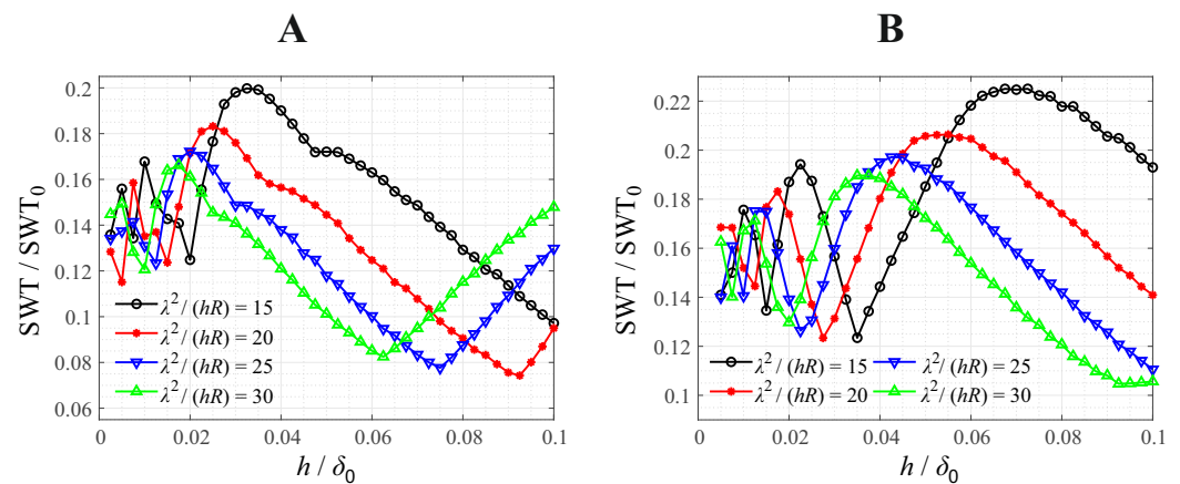
Figure 7. Normalized maximum SWT parameter for the same-frequency bimodal contact oscillation between a paraboloid with small waviness and a flat, as a function of the normalized waviness amplitude, for different values of the normalized wave length; (A): for \delta_A = 0.25 \delta_0 ; (B): for \delta_A = 0.75 \delta_0 .
